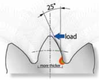
Pressure Angle 25° (Sumitomo PARAMAX ® Series)
