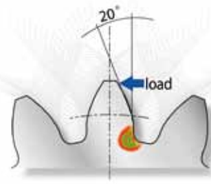
Pressure Angle 20° (Conventional Gears)
