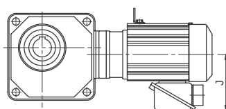
Fig. 6 Without brake
