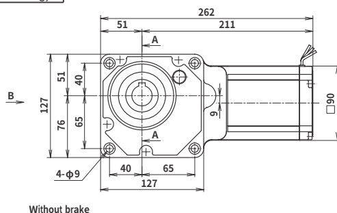
Without brake
