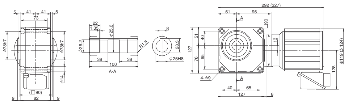
Fig. 4 Designate model and voltage and frequency when ordering. Brackets contain dimension, model, or mass of type with brakes. RNYM01-1230-80-240 Mass 7.5kg (RNYM01-1230-B-80-840) (Mass 9.0kg)
