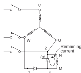
Fig. 15 standard circuit
