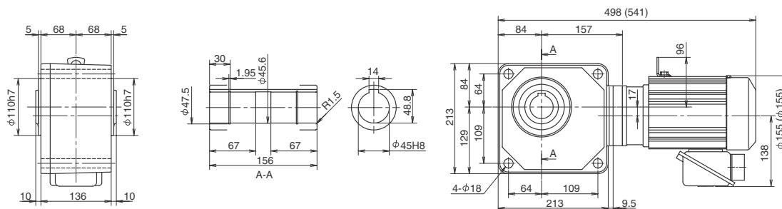
Fig. 4 Designate model and voltage and frequency when ordering. Brackets contain dimension, model, or mass of type with brakes. RNYM08-1530-80~240 Mass 24kg (RNYM08-1530-B-80~240) (Mass 26kg)
