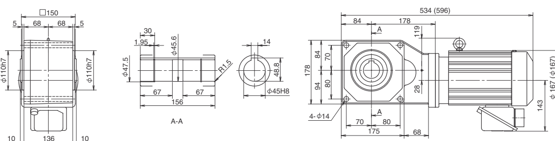
Fig. 3 RNYM1H-1520-40~60 (RNYM1H-1520-B-40~60) Mass 29kg (Mass 33kg)
